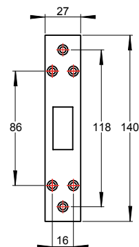
Deadbolt/Sliding Lock Strike MLPA5100-02
